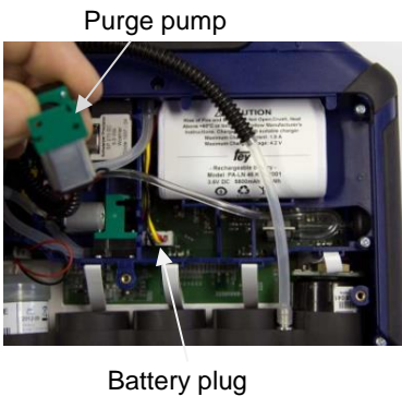
Fig. 74: Before exchanging the battery remove the purge pump
