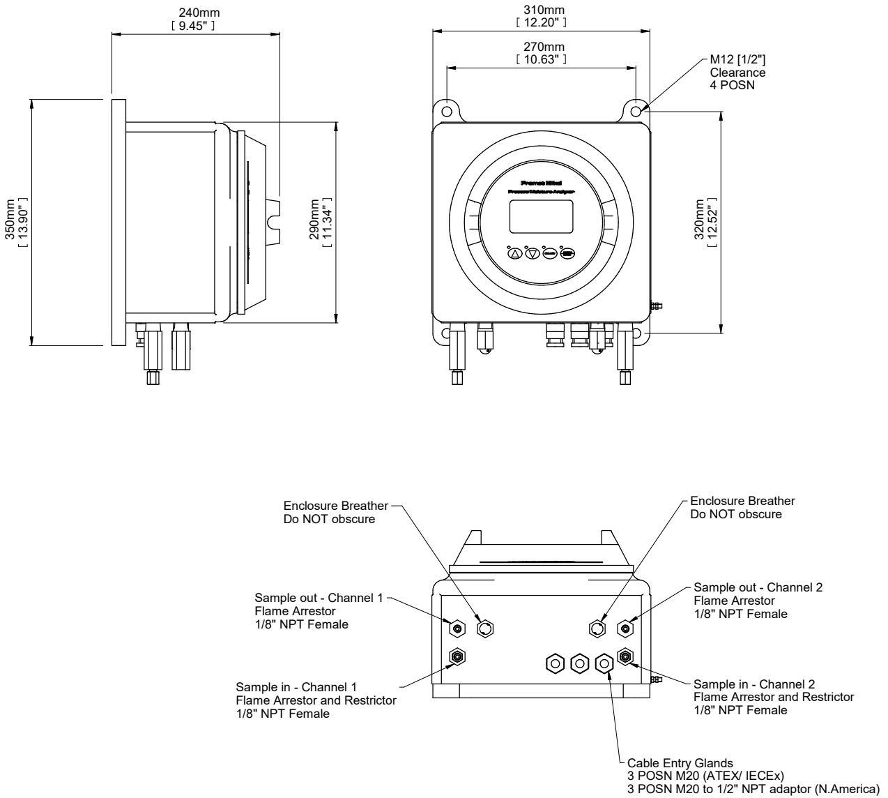
Figure 27 Mounting Drawing
