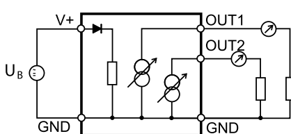
Schematic 3-wire type (current signal)
