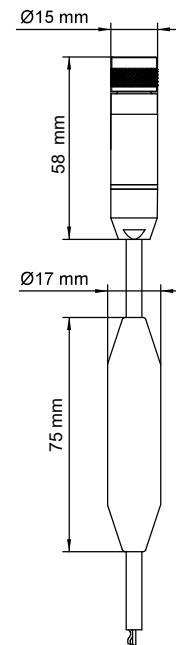
AC3003
